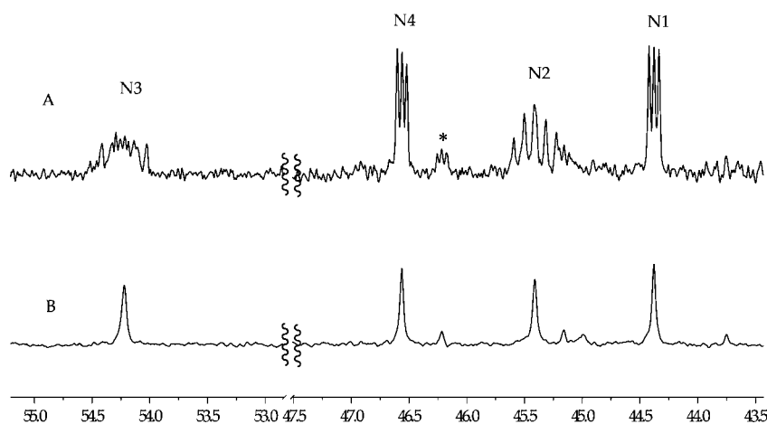
Figure 3. ^{15}\text{N} NMR spectra of 0.10 M [\text{}^6\text{Li}, \text{}^{15}\text{N}]\mathbf{6} prepared from [\text{}^{15}\text{N}_4]\mathbf{3} with 4.0 equiv of n -BuLi in 6.10 M THF/pentane recorded at -90\text{ }^\circ\text{C} after aging at -78\text{ }^\circ\text{C} overnight: (A) fully coupled and (B) broadband ^{15}\text{N} decoupled. * indicates unknown impurities that appear sporadically.
