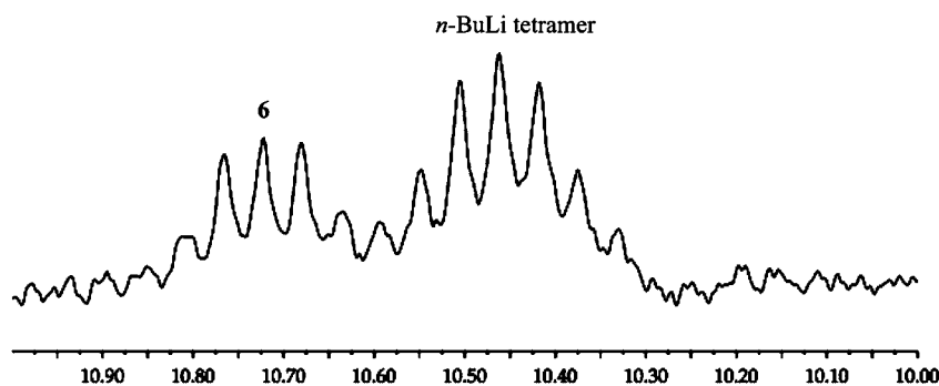
Figure 4. ^{13}\text{C} NMR spectra of 0.10 M [\text{Li}_4^{15}\text{N}]_6 prepared from [\text{N}_4^{15}]_3 with 4.0 equiv of n -BuLi in 6.10 M THF/pentane recorded at -90 °C after aging at -78 °C overnight. The ^{13}\text{C} resonance of the n -BuLi dimer is not shown but appears as a 1:2:3:2:1 quintet at 12.6 ppm.
