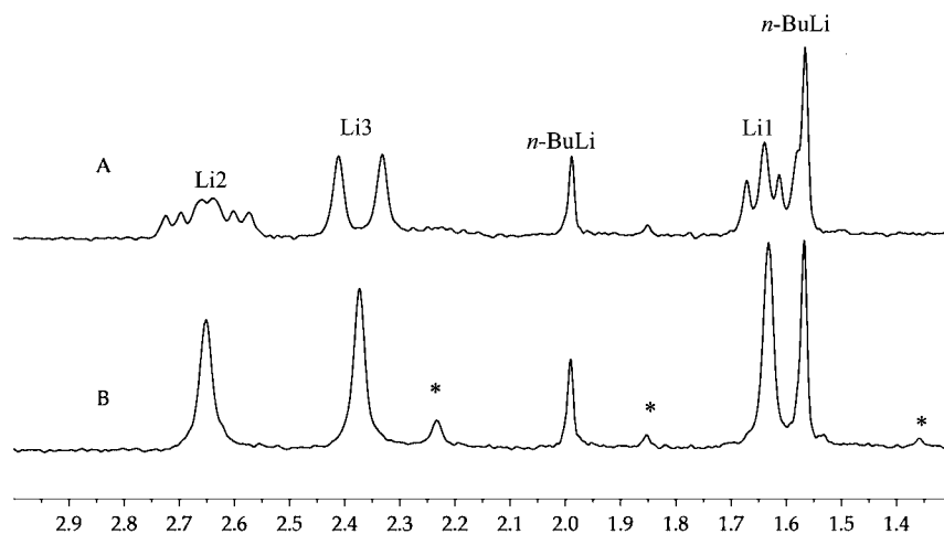
Figure 2. ^6\text{Li} NMR spectra of 0.10 M [\text{}^6\text{Li}, \text{}^{15}\text{N}]\mathbf{6} prepared from [\text{}^{15}\text{N}_4]\mathbf{3} with 4.0 equiv of n -BuLi in 6.10 M THF/pentane recorded at -90\text{ }^\circ\text{C} after aging at -78\text{ }^\circ\text{C} for 2.0 h: (A) fully coupled and (B) broadband ^{15}\text{N} decoupled. * indicates unknown impurities that appear sporadically.
